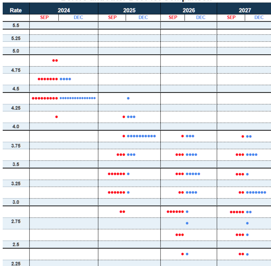
Before and After Dot Plot Comparison
